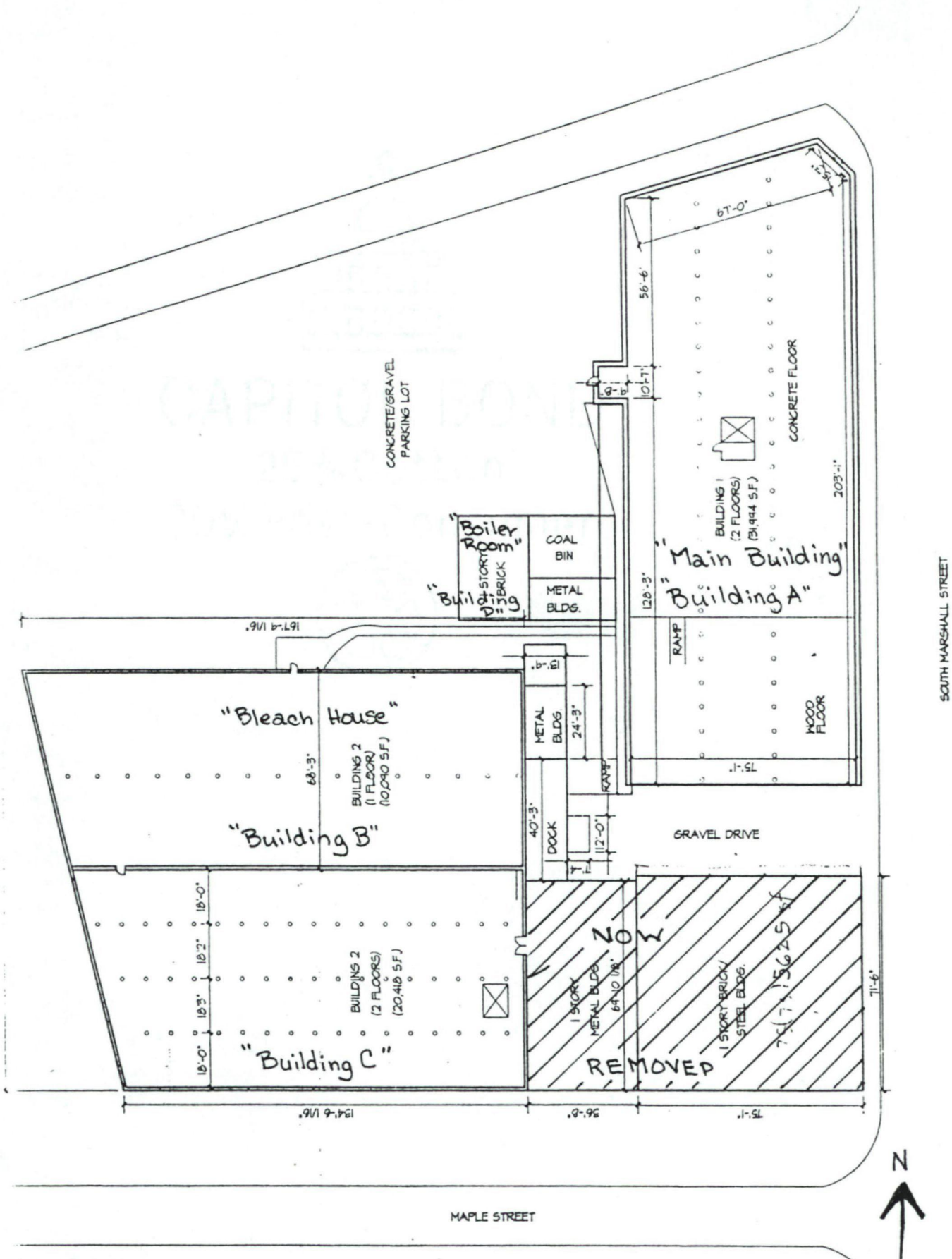
INDERA MILLS FORSYTH CTY., NC Exhibit 3: Plan of Indera Mills Complex June 18, 1997
